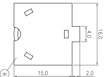
VIEW WITH COVER
