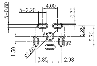
RECOMMEND P.C.B LAYOUT TOP VIEW(TOLERANCES:±0.05)
