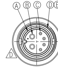
F CONN M PIN WATERPROOF RATE: IP67
